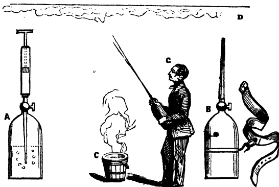
Fig. 172. A. Section of copper bottle with pipe, condensing pump, and stopcock. The bottle is half full of the alcoholic solution. B. Copper bottle ready for use, with the jet screwed on and attached to a leathern belt by a ring and hook. C. Pail of boiling water. G. Use of the copper bottle, from which the jet of alcohol escapes to the ceiling D, where a torch of tow dipped in spirits of wine is held for a few minutes, till it takes fire properly.
